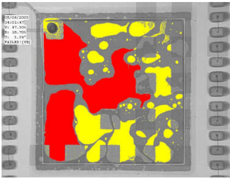
Figure 2b. – Example of die attach void analysis. Yellow and red coloring are used to differentiate void areas & densities in this example.
