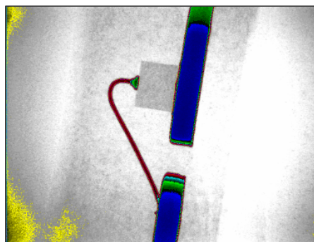
Figure 2a. – Example of bond wire inspection. Gray Scale Densities are converted to color for analysis in this example.
