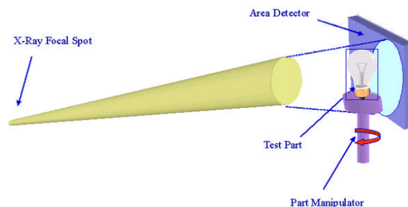
Figure 7 – Cone Beam Method Illustration
