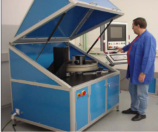
Fig. 6: Automatic shearography system for abrasion-resistant seals inspection.
